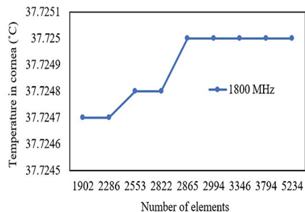
Fig. 5 Grid convergence graph between number of mesh elements and temperature.
