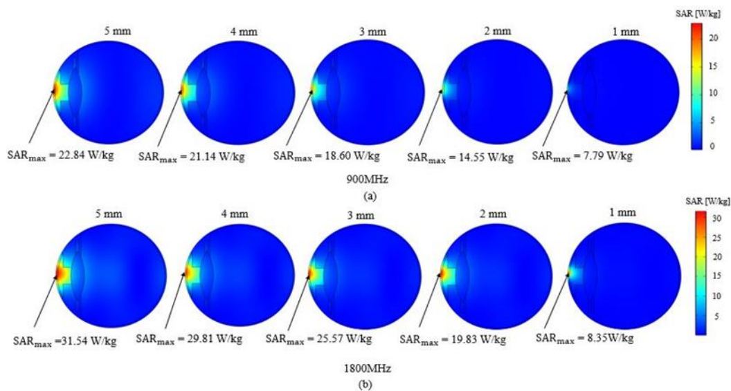
Fig. 11 Comparison of different sizes of electromagnetic source on the SAR in the eye at 317 sec position for (a) 900 MHz, and (b) 1800 MHz frequencies.
