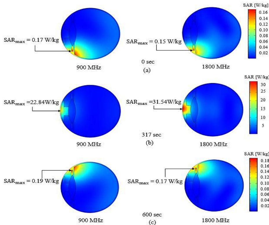
Fig. 9 SAR distribution in the eye at (a) 0 sec, (b) 317 sec, and (c) 600 sec.
