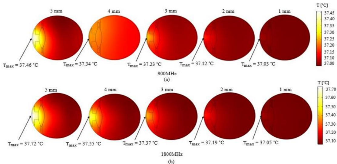
Fig. 12 Comparison of different sizes of EM source on the temperature in the eye at 317 sec position for (a) 900 MHz, and (b) 1800 MHz frequencies.
