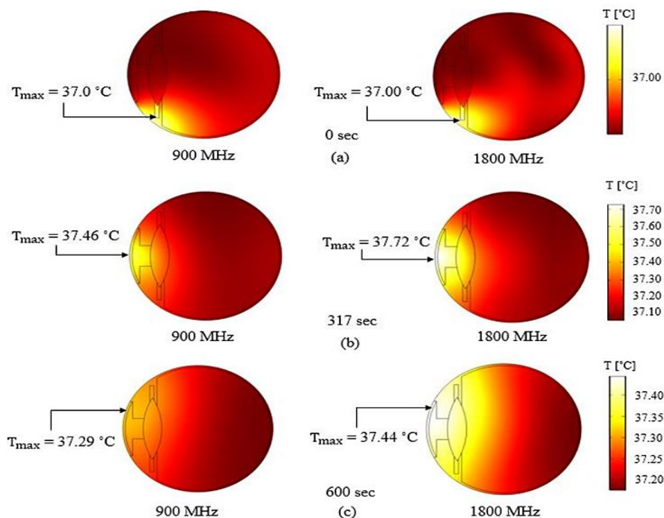
Fig. 10 Temperature distribution in the eye at (a) 0 sec, (b) 317 sec, and (c) 600 sec.
