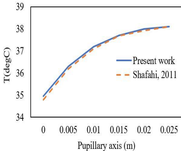
Fig. 6 Comparison of the temperature distribution inside the eye between present work and the work of Shafahi and Vafai. [33]
