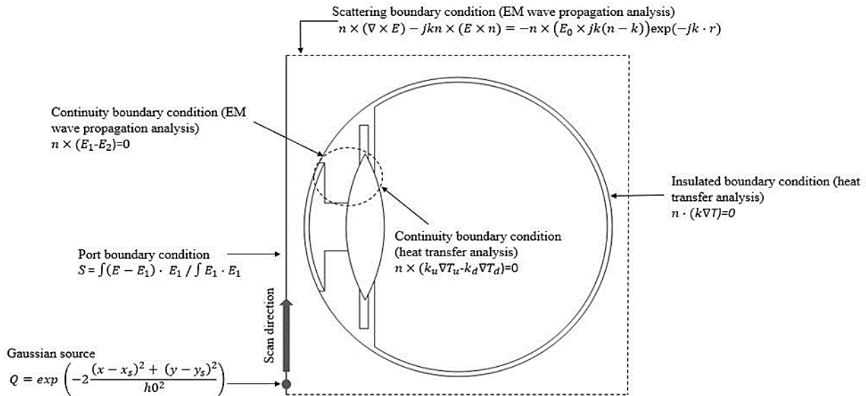
Fig. 3 Boundary condition for electromagnetic wave propagation and bio-heat transfer analysis.
