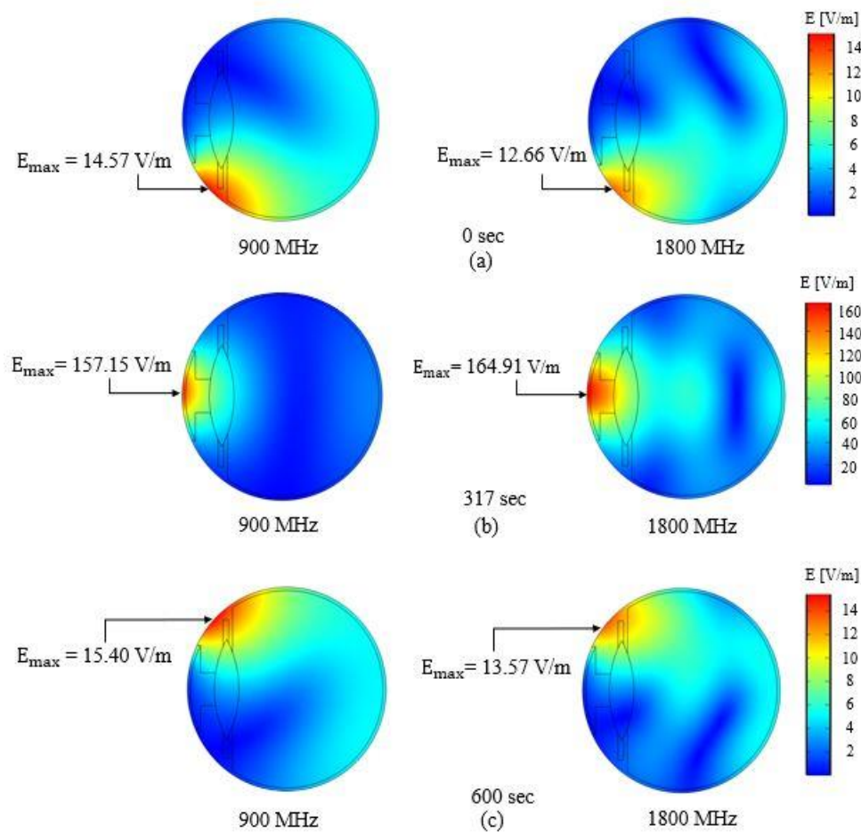
Fig. 8 Electric field distribution in the eye at (a) 0 sec, (b) 317 sec, and (c) 600 sec.
